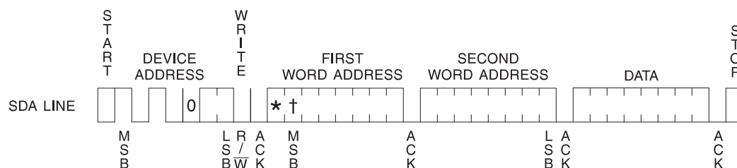
Figure 8. Byte Write
