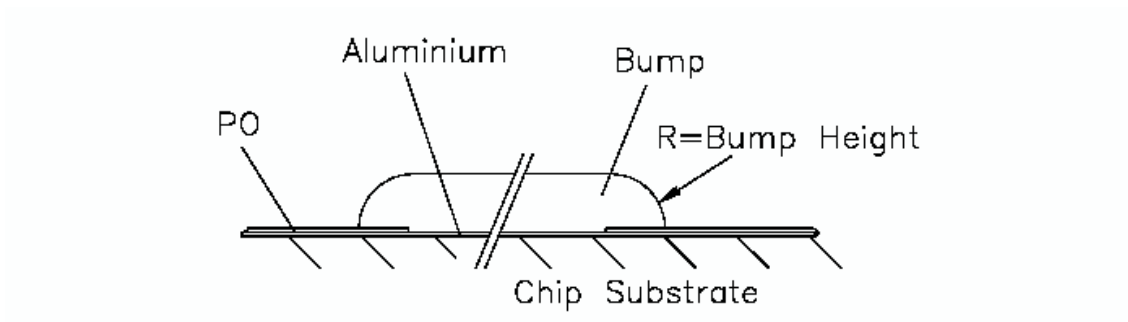
Figure 2-3. Cross Section of Bump
