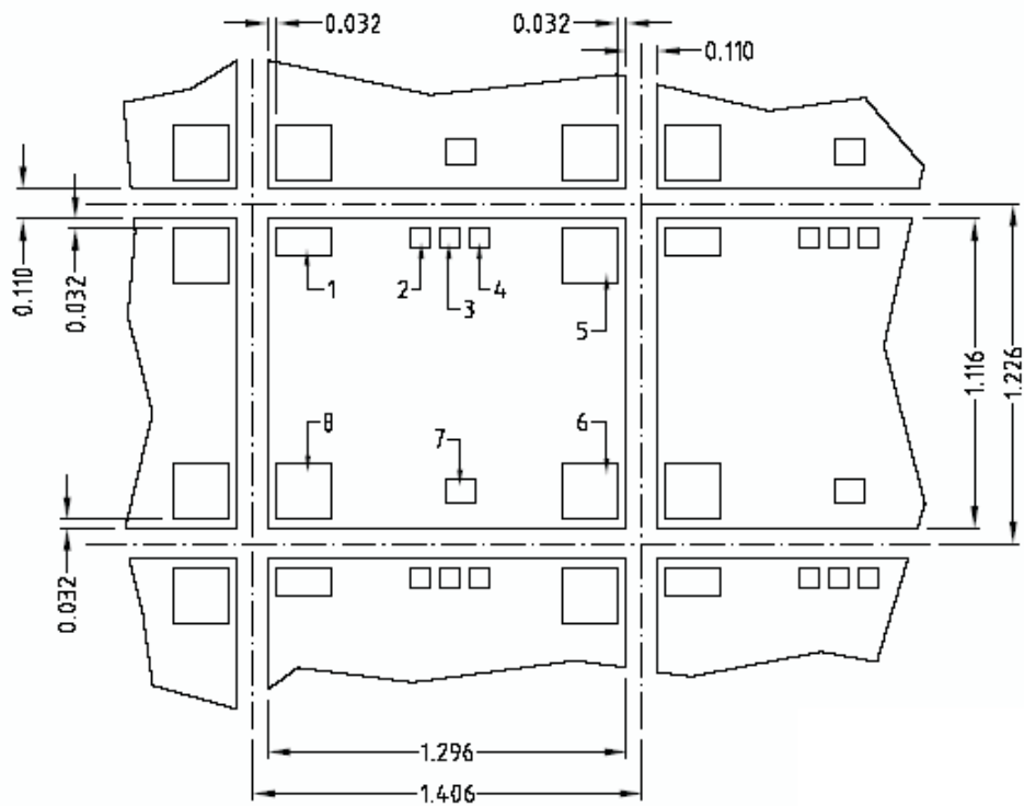
Figure 2-2. Antenna and Test Pad Location
